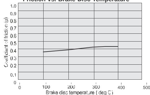
Standard MC, Organic Asbestos free Friction vs. Brake Disc Temperature
