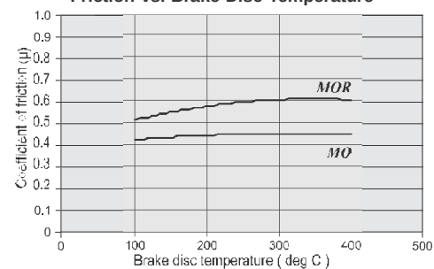
MX / ATV, Sinter Metallic • Standard & Racing Friction vs. Brake Disc Temperature
