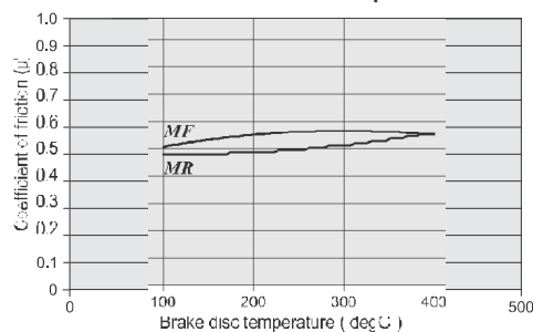
Supersport MC, Sinter Metallic Friction vs. Brake Disc Temperature
